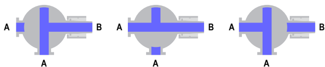
CX-092 Three position valve with two female luer ports (A) and one male luer lock (B)
