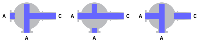
CX-093 Three position valve with two female luer ports (A) and one male slip luer port (C)
