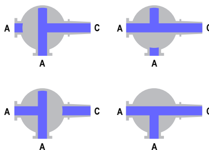
CX-094 Four position valve with two female luer ports (A) and one male slip luer port (C)
