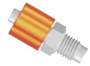
CX-045 Male Rotating Lock Ring Luer to 1/4-28 Thread
