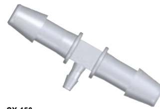
CX-156 T Shaped 3/32" (1) to 1/4" (2) Barbs
